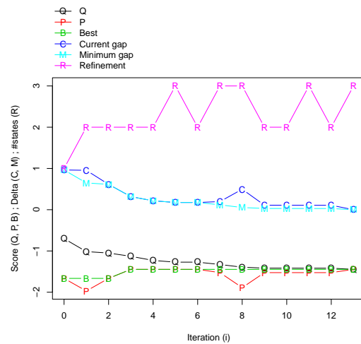
Figure 1: Certificate of optimality.
