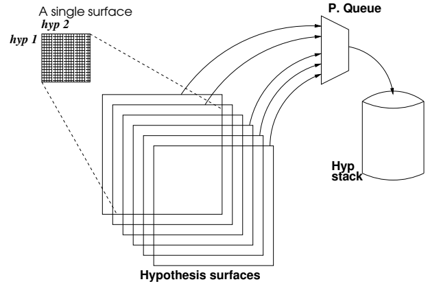
Figure 1: Illustration of Lazier Cube Pruning
